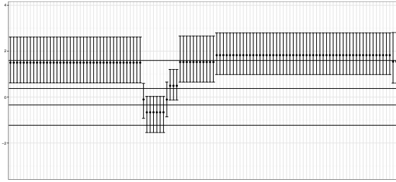
(b) Posterior median and 95 percent HPD interval, model with vague prior
